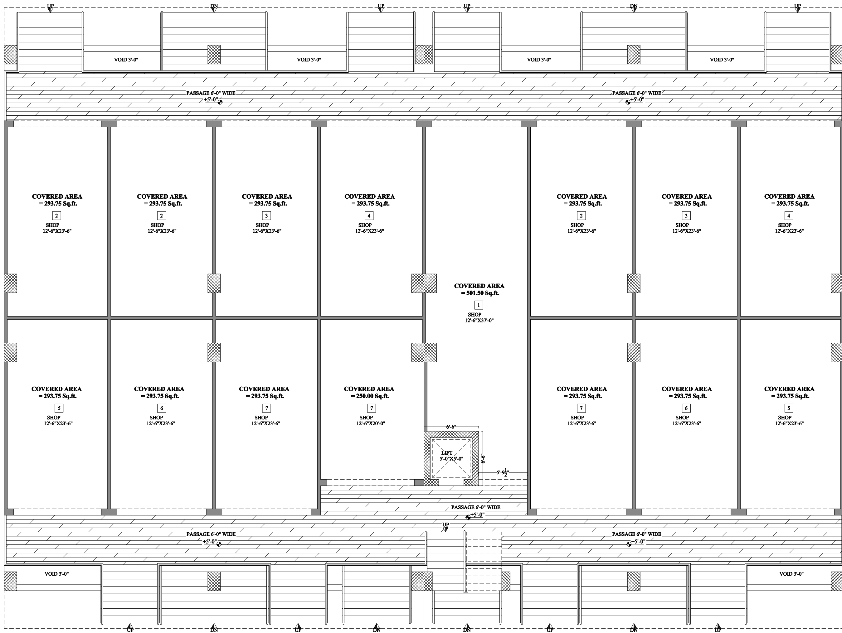
GROUND FLOOR PLAN COVERED AREA = 6500.00 Sq.ft. NOTE:- ALL DIMENSION INCLUDING WALLS
