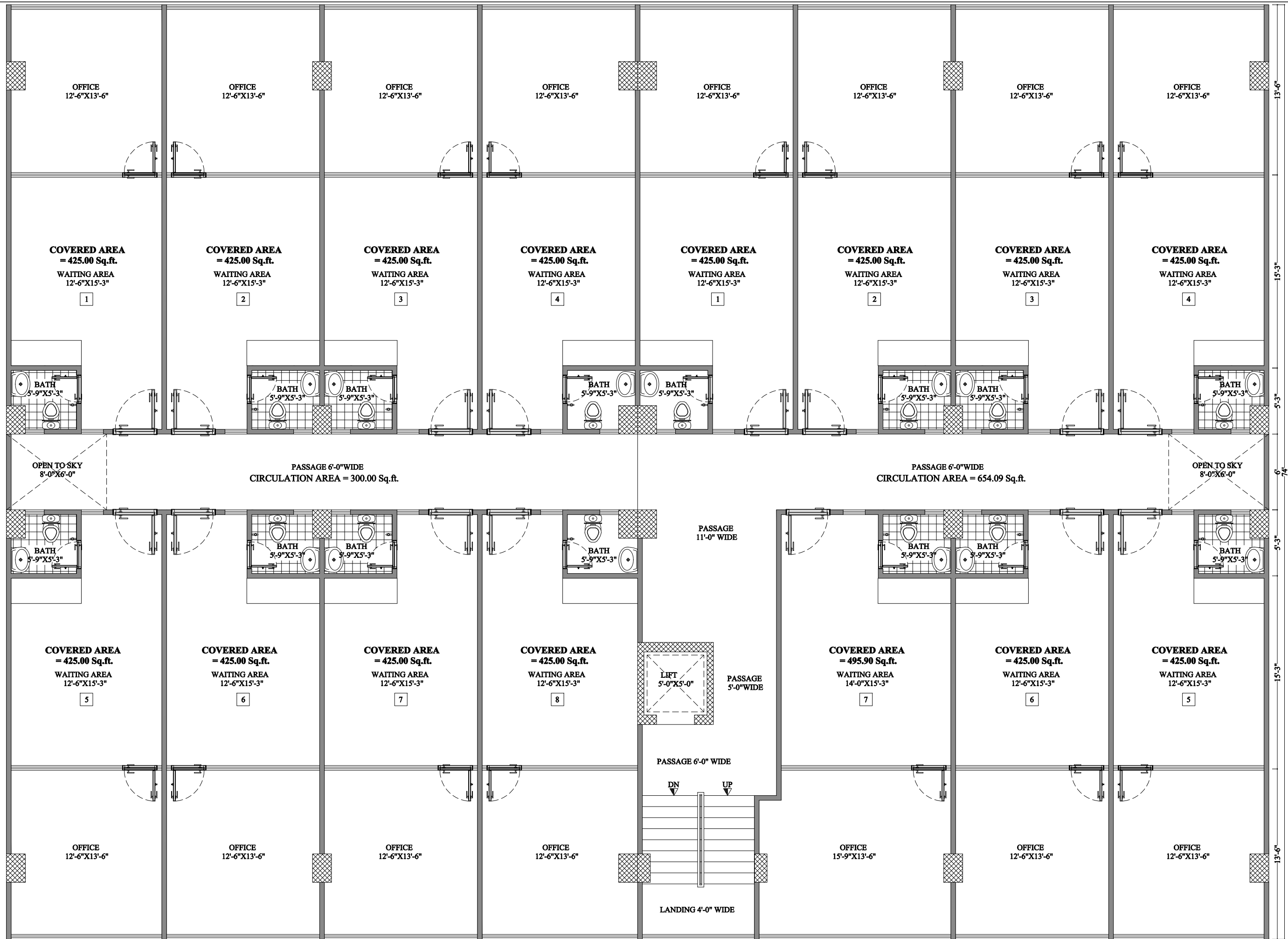
1st & 2nd FLOOR PLAN COVERED AREA = 7400.00 Sq.ft. NOTE:- COVERED AREA WITH CIRCULATION NOTE:- ALL DIMENSION INCLUDING WALLS
